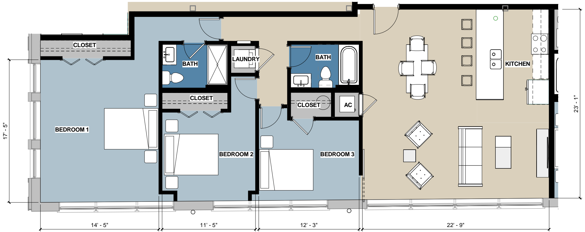
UNIT 302 = 1504 GSF
